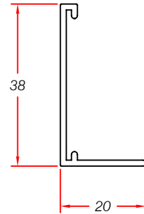
ET180 EXTRUDED ANGLE
