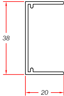
ET181 EXTRUDED CHANNEL
