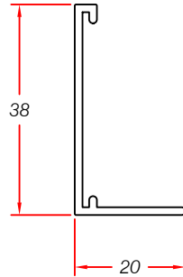
ET180 EXTRUDED ANGLE
